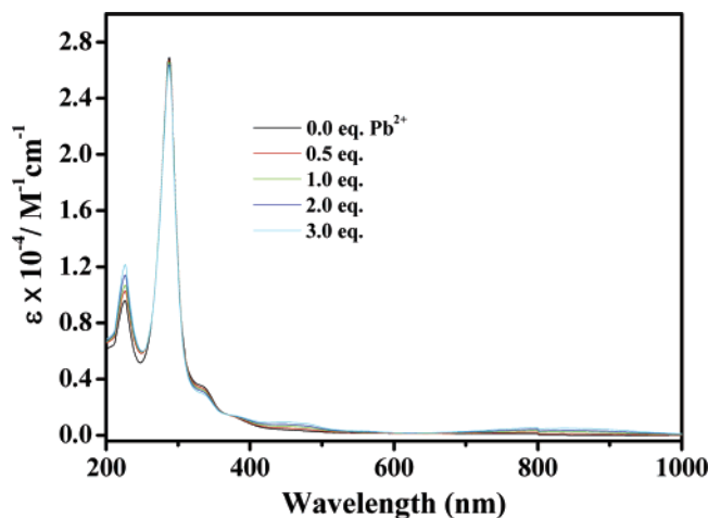
Figure 7. Absorption spectra (with an \epsilon scale) of dyad 3 recorded in a mixture of CH 2 Cl 2 and CH 3 CN (1:1, v/v; 5.0 × 10 -5 M) in the presence of increasing amounts of Pb 2+ [Pb(ClO 4 ) 2 ].
