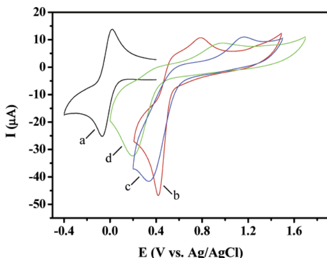
Figure 8. Cyclic voltammograms of compound 5 (2.0 × 10 -3 M) before (a, black) and after addition of 4.0 equiv of Pb(ClO 4 ) 2 (b, red), Sc(SO 3 -CF 3 ) 3 (c, blue), and Zn(ClO 4 ) 2 (d, green) in CH 2 Cl 2 /CH 3 CN (1:1, v/v) at a scan rate of 100 mV s -1 .
