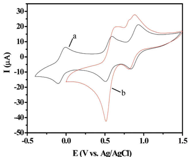
Figure 9. Cyclic voltammograms of dyad 1 (1.0 × 10 -3 M) (a, black) before and (b, red) after addition of 2.0 equiv of Pb(ClO 4 ) 2 in CH 2 Cl 2 /CH 3 CN (1:1, v/v) at a scan rate of 100 mV s -1 .
